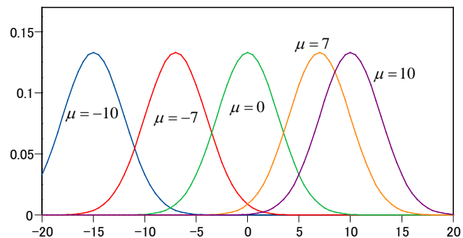
Figure 1 Probability density functions of Normal Distribution
